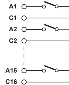
40-137-001 5A Power Relay Module - 16 x SPST
