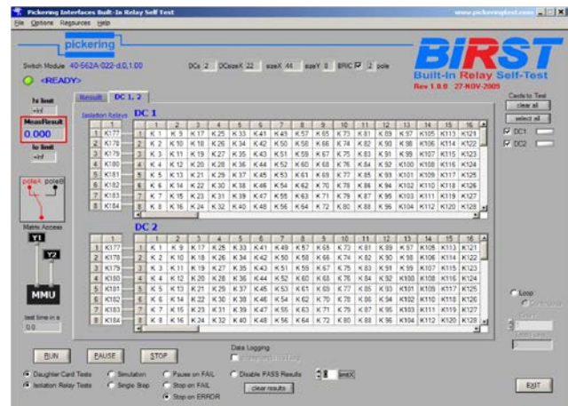
Test Sequencer Front Panel for BIRST. This allows any combination of tests to be run in either single or multiple sequences. All test data is displayed in the results window and can be written to a data file.
