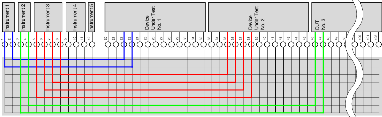
Schematic diagram showing a 192x8 BRIC Matrix being used to parallel test multiple DUTs. The BRIC Matrix allows tremendous test system flexibility.
