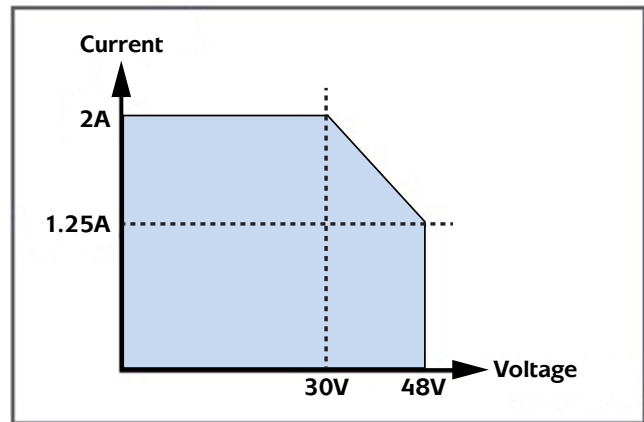
41-740 Safe Operational Area
