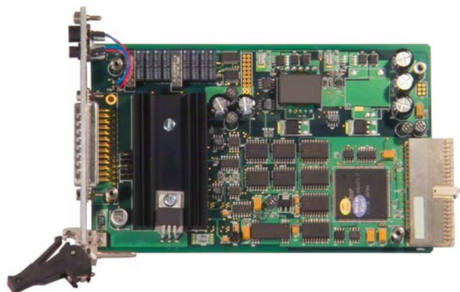
41-751 PCB View
