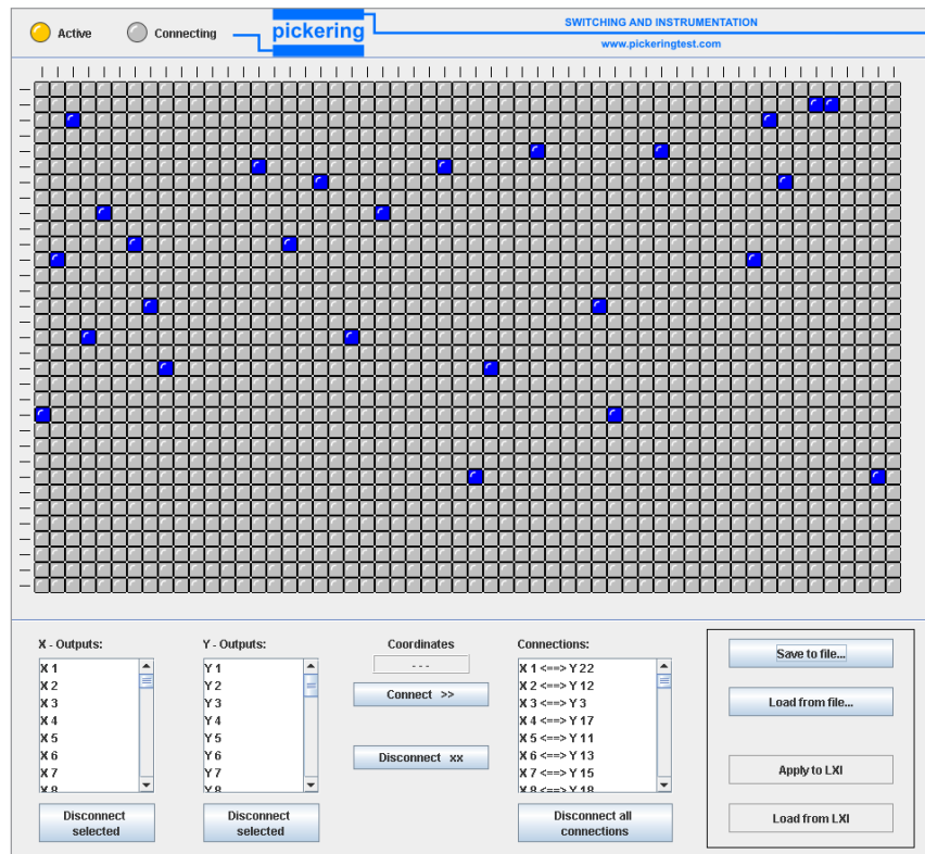
Soft Front Panel for the 60-510 LXI Low Thermal EMF Matrix
