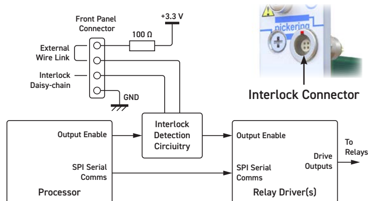
Interlock Signal Routing Diagram for 40-182A Versions With Hardware Interlock Option
