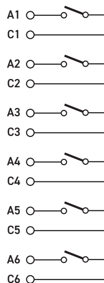
40-182A-011 Solid State Switch - 6 x SPST
