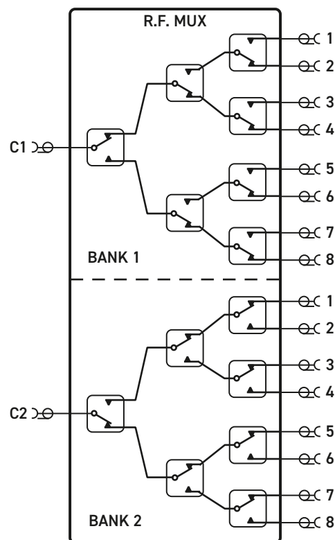
Dual 8 to 1 RF MUX (Part No. 4x-834A-x02) Default Switch Paths Shown
