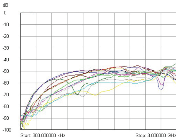
Typical Crosstalk Between Channels (these are measurements of crosstalk within each multiplexer for neighboring channels).
