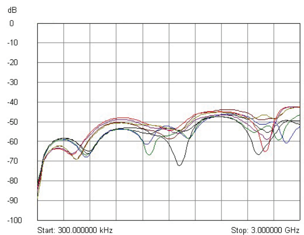
Typical Crosstalk Between MUX Banks (these are measurements of crosstalk between the same paths through neighboring multiplexers).
