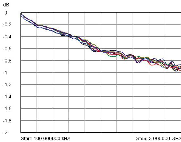
Typical Insertion Loss Plot
