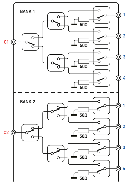
Dual 4 to 1 Terminated RF MUX (Part No. 40/42-873A-x02) Default Switch Paths Shown
