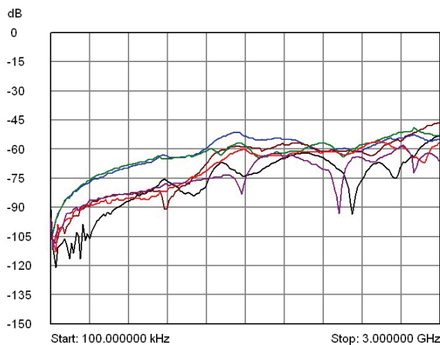
Typical Crosstalk Plot - Channel to Channel
