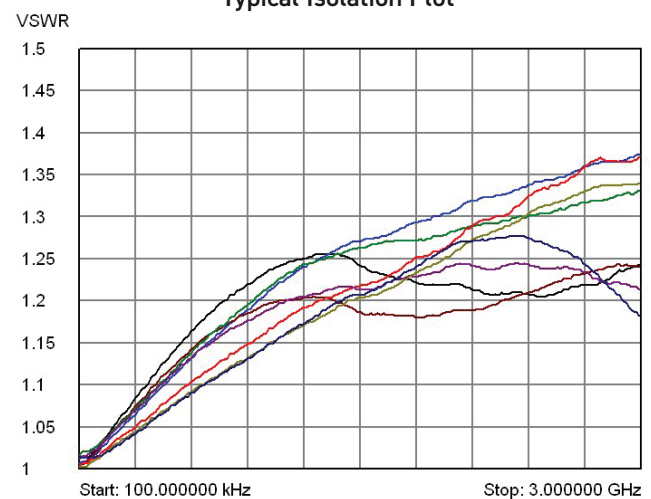
Typical VSWR Plot - Terminated
