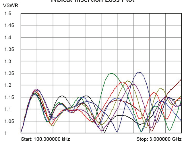
Typical VSWR Plot - Signal Paths
