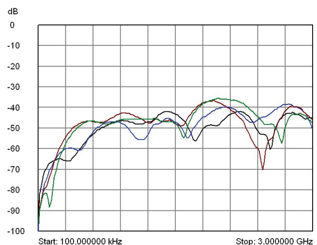
Typical Crosstalk Plot - Bank to Bank
