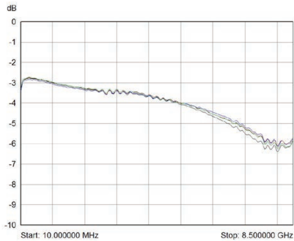
Insertion loss for 4x-882B-001 showing all paths up to 8.5 GHz
