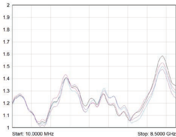
VSWR COM to Channel for 4x-882B-001 showing all paths up to 8.5 GHz
