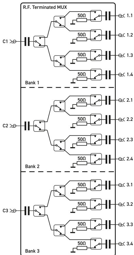
Triple SP4T Terminated 8 GHz MUX (Part No. 4x-882B-003)
