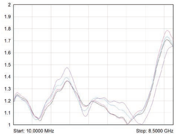
VSWR Channel to COM for 4x-882B-001 showing all paths up to 8.5 GHz
