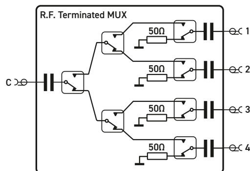
Single SP4T Terminated 8 GHz MUX (Part No. 4x-882B-001)
