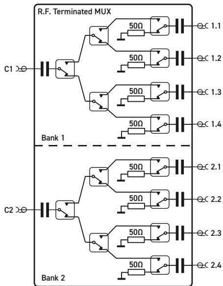
Dual SP4T Terminated 8 GHz MUX (Part No. 4x-882B-002)
