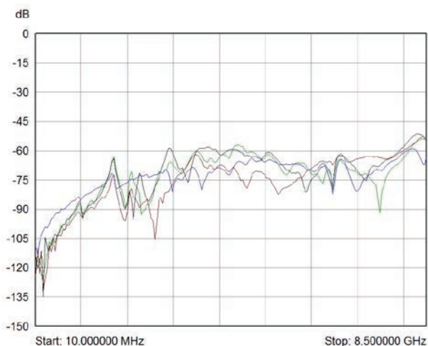
Max isolation for each channel with distant path selected for 4x-882B-001 up to 8.5 GHz
