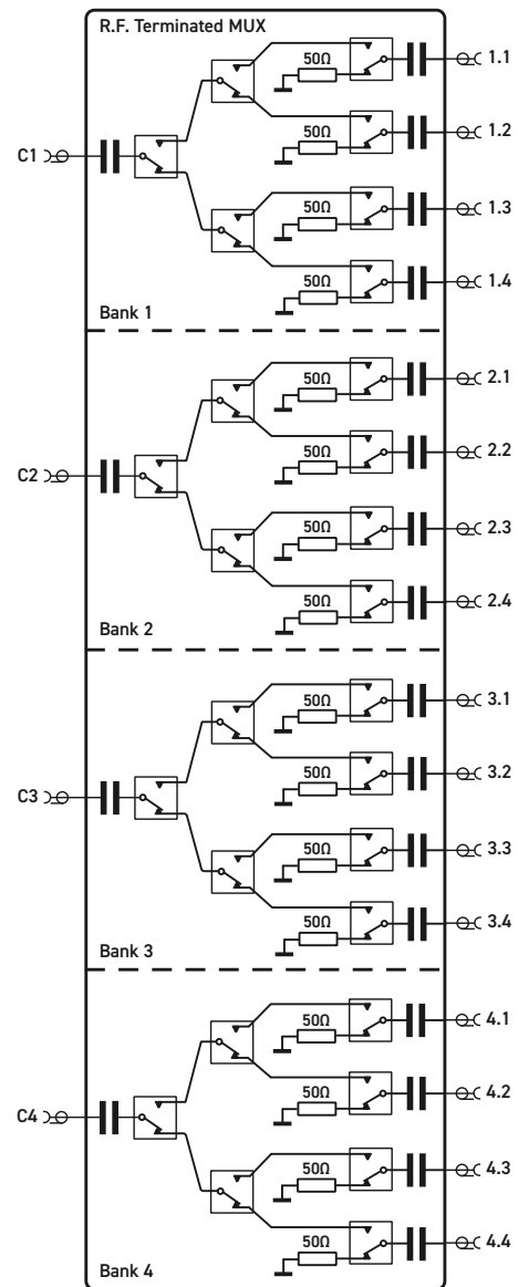
Quad SP4T Terminated 8 GHz MUX (Part No. 4x-882B-004)
