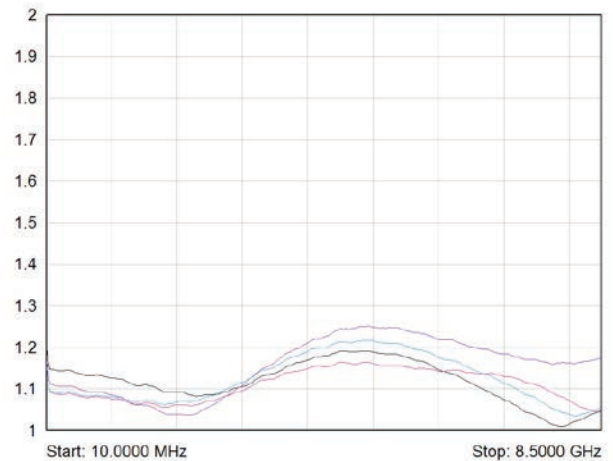
VSWR Terminated Channel for 4x-882B-001 showing all paths up to 8.5 GHz
