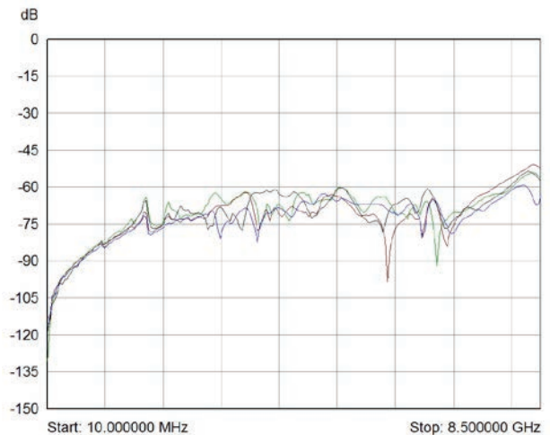
Crosstalk between adjacent channels for 4x-882B-001 showing all paths up to 8.5 GHz
