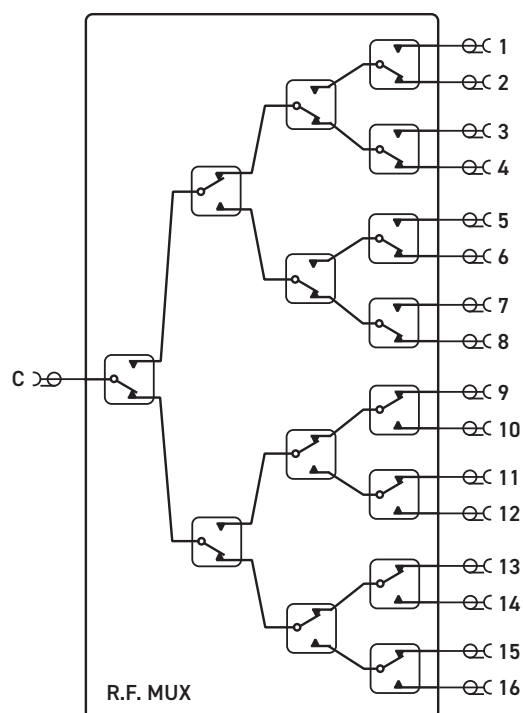
40-875 16 to 1 RF MUX Functional Diagram (Default Switch Paths Shown)
