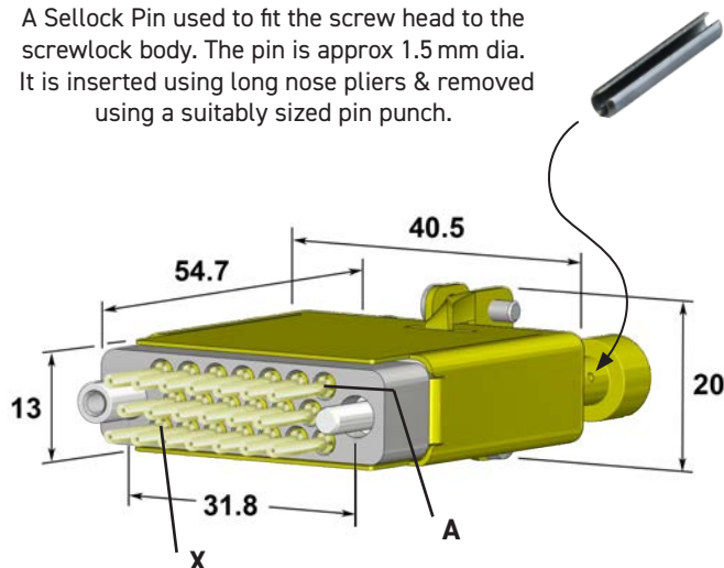
Connector Dimensions
