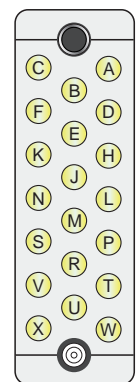
End A - Male Mating Face
