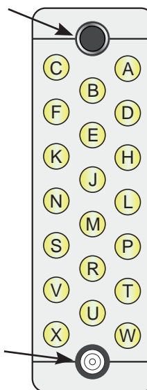
Rear View of Connector (Without Pins Fitted)
