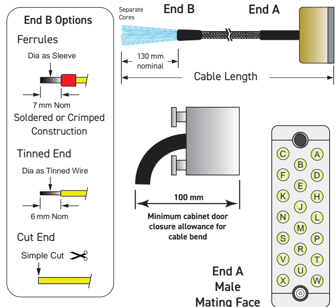
10 A 20-Pin GMCT Underterminated Cable Assy
