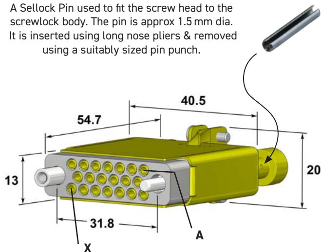
Connector Dimensions
