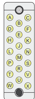
End A - Female Mating Face
