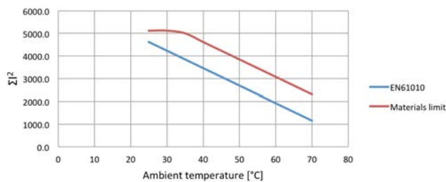
Characteristic Plots for 40-970B-020-1m
