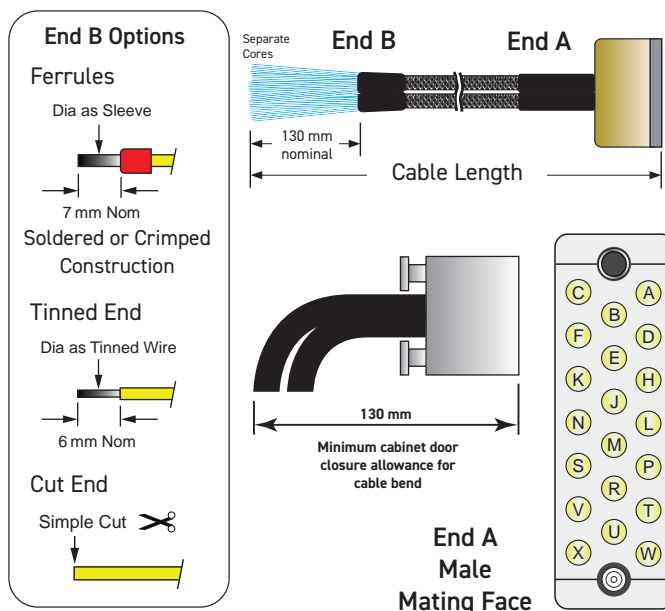
16 A 20-Pin GMCT Unterminated Cable Assy
