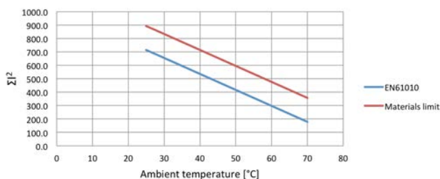
Characteristic Plots for A020GMR-A020GMR-0B100
